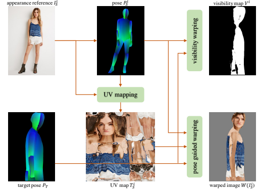
Figure 4. 3D-aware warping in UV space. The goal is to warp i^{th} source image I_S^i to the target pose P_T . First, based on the correspondence between the estimated source pose P_S^i and target pose P_T , the visibility map V_i is computed. Then, based on the source pose P_S^i , the source image I_S^i is mapped to the UV-space, and inpainted to obtain the UV texture map T_S^i . UV map can be mapped to 2D W(I_S^i) , which is the warped image. W(I_S^i) and V_i are later used for multi-view fusion.
