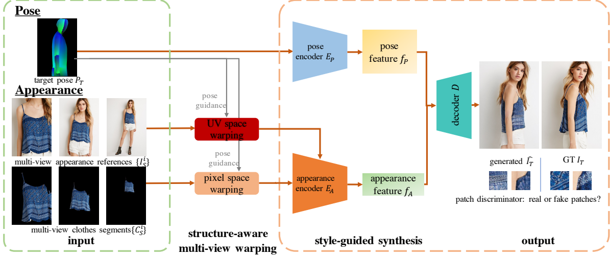
Figure 2. Overview of our method for human reposing. We take a pose image P_T as the reference for the target human pose, as well as multi-view human images \{I_S^i\} as the reference for the target human appearance, i.e., the face identity, the skin tone and the garment texture. Pose reference P_T is fed to the pose encoder E_P for the pose feature f_P . Appearance reference images \{I_S^i\} and their corresponding garment segments \{C_S^i\} are warped to the target pose in both UV and pixel space (Section 3.1), and encoded as an appearance features \{f_A^i\} with the appearance encoder E_A . \{f_A^i\} of every view is fused to an aggregated appearance feature f_A based on visibility from each source to the target pose (Section 3.2). The StyleGAN2-based [18] decoder D takes the structure and the appearance feature f_P, f_A and decodes them as the output image \hat{I}_T . To improve the synthesis quality, we supplement a conditional patch discriminator to the generative adversarial networks (Section 3.3). The method could be easily adapted for virtual try-on during inference.
